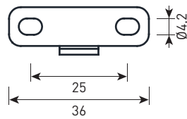
Bracket SIZE 1
