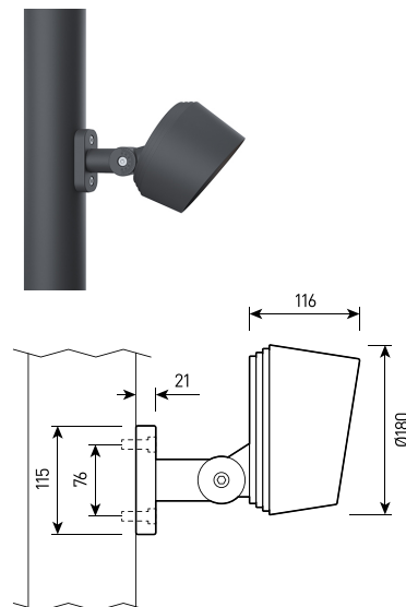
4 bracket to pipe
