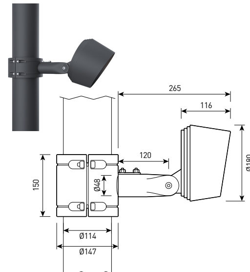
5 wrap-around bracket
