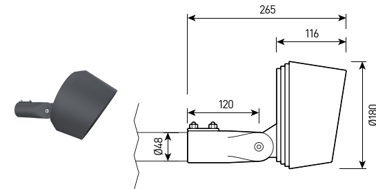
3 pipe mount
