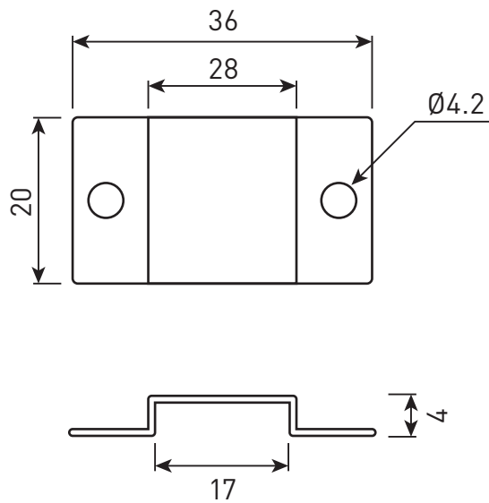
Stainless steel wire clamp
